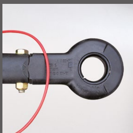
DIN towing eye for height-adjustable drawbar, 2000-2500 kg and 3000-3500 kg
